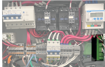
Three-phase EI Link
